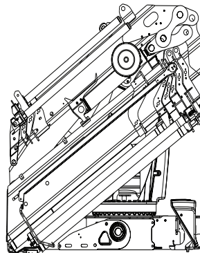
X-HiPro 358-5 + Jib 100X-2 Front View
